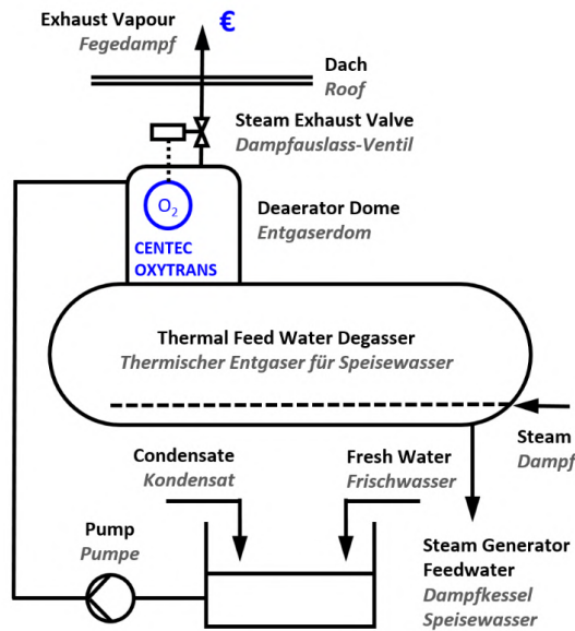
Fig. 4 Schematic Structure of the Process
